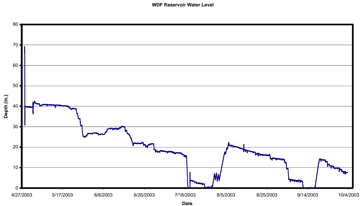
Figure 6. WDF Reservoir Water Level Graph.
