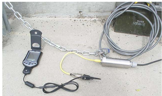
Figure 5. Telog PR-31 connected to the M125 Palm Pilot.
