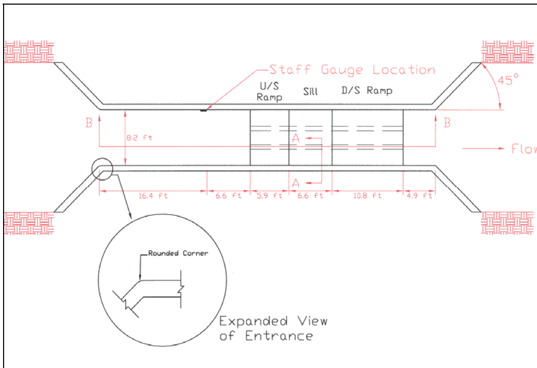
Figure 7. AutoCAD plan view drawing of rectangular Replogle flume installation with recommended entrance and exit conditions
