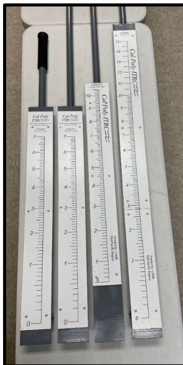
FACEPLATES FROM LEFT TO RIGHT: 7 CFS/ft, 7 CFS/ft, 10 CFS/ft, 15 CFS/ft
