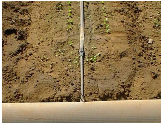
Figure 2. Manifold connection with layflat hose, a short (30 cm) section of PE hose, and "quick release" fittings on both ends of the PE hose section.
