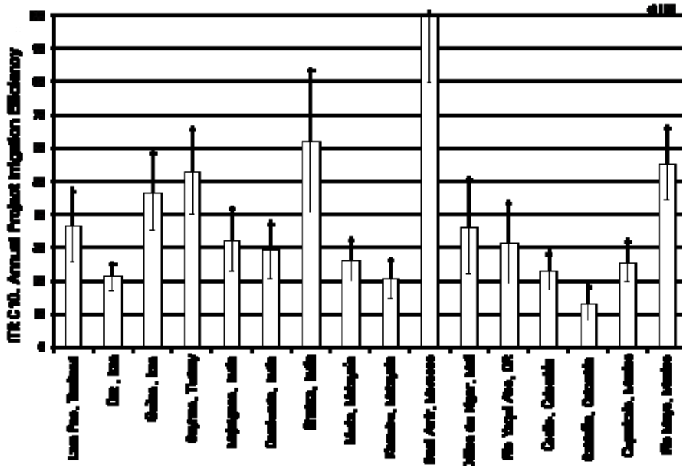
Figure 7. Project Annual Irrigation Efficiency.
