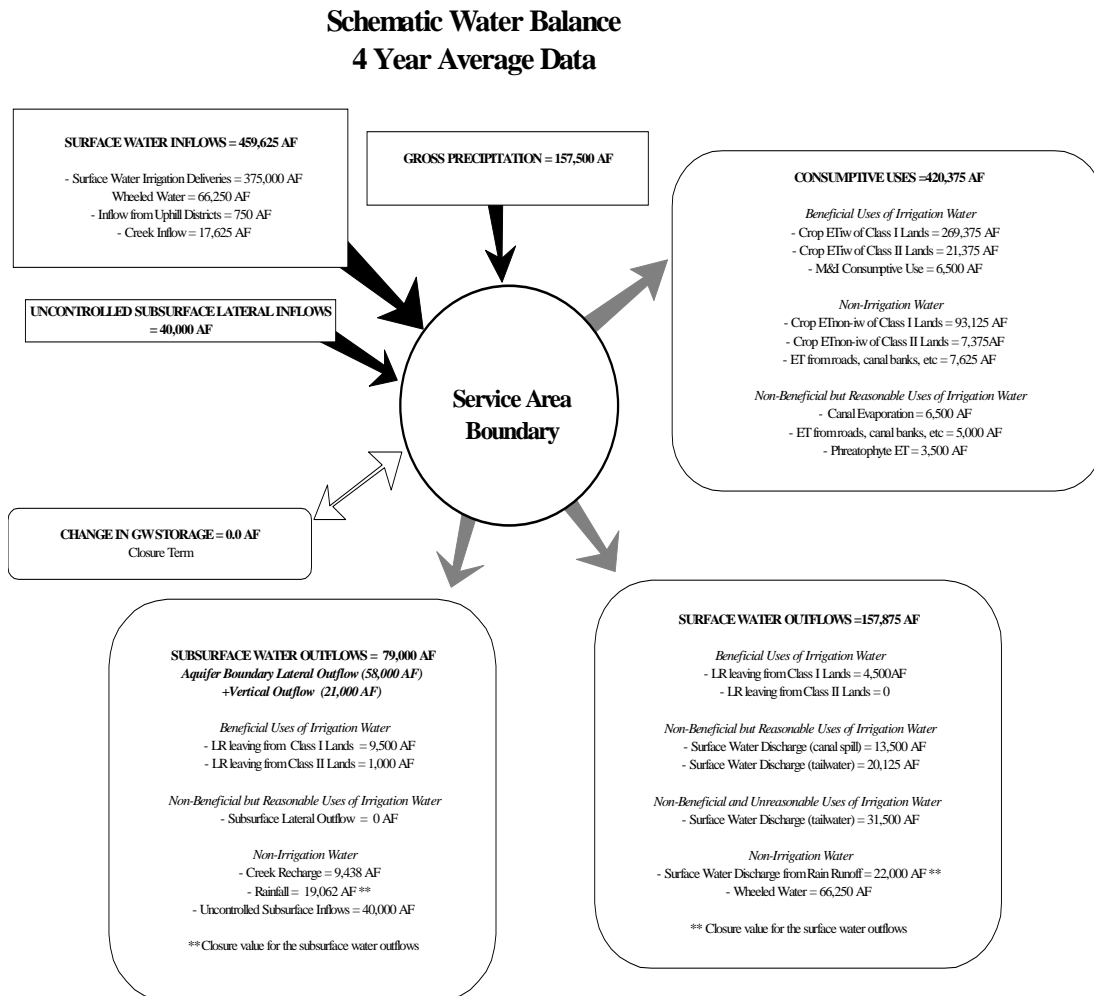
Fig. 2. Schematic of Detailed Water Balance (from Styles and Burt, 1998).
