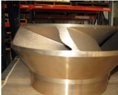
Figure 4. The thickness on the bottom of the vane is correct; the thickness must be reduced on the upper portion of the vane.
