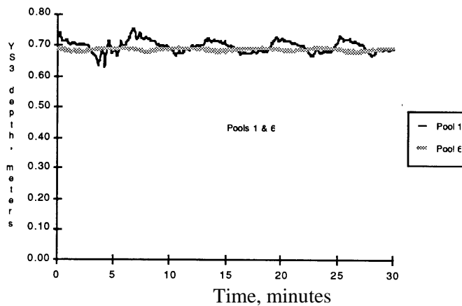
Figure 4. Results of a test with multiple turnout flow rate changes. Conducted on the physical canal.
