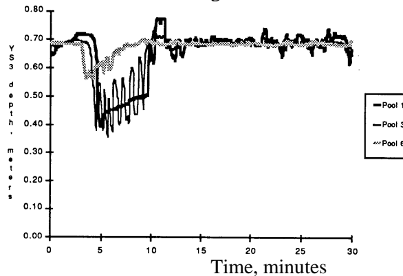
Figure 6. Results of instantaneous flow rate change of 113 \text{ m}^3\text{h}^{-1} to 340\text{m}^3\text{h}^{-1} at far downstream end of the model canal. Conducted on the physical model canal.
