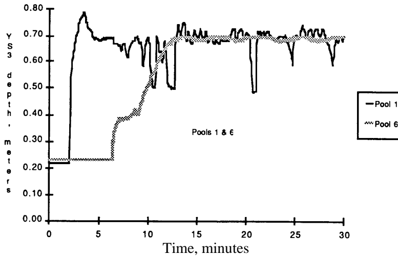
Figure 5. Startup of the physical model canal from a dry condition.
